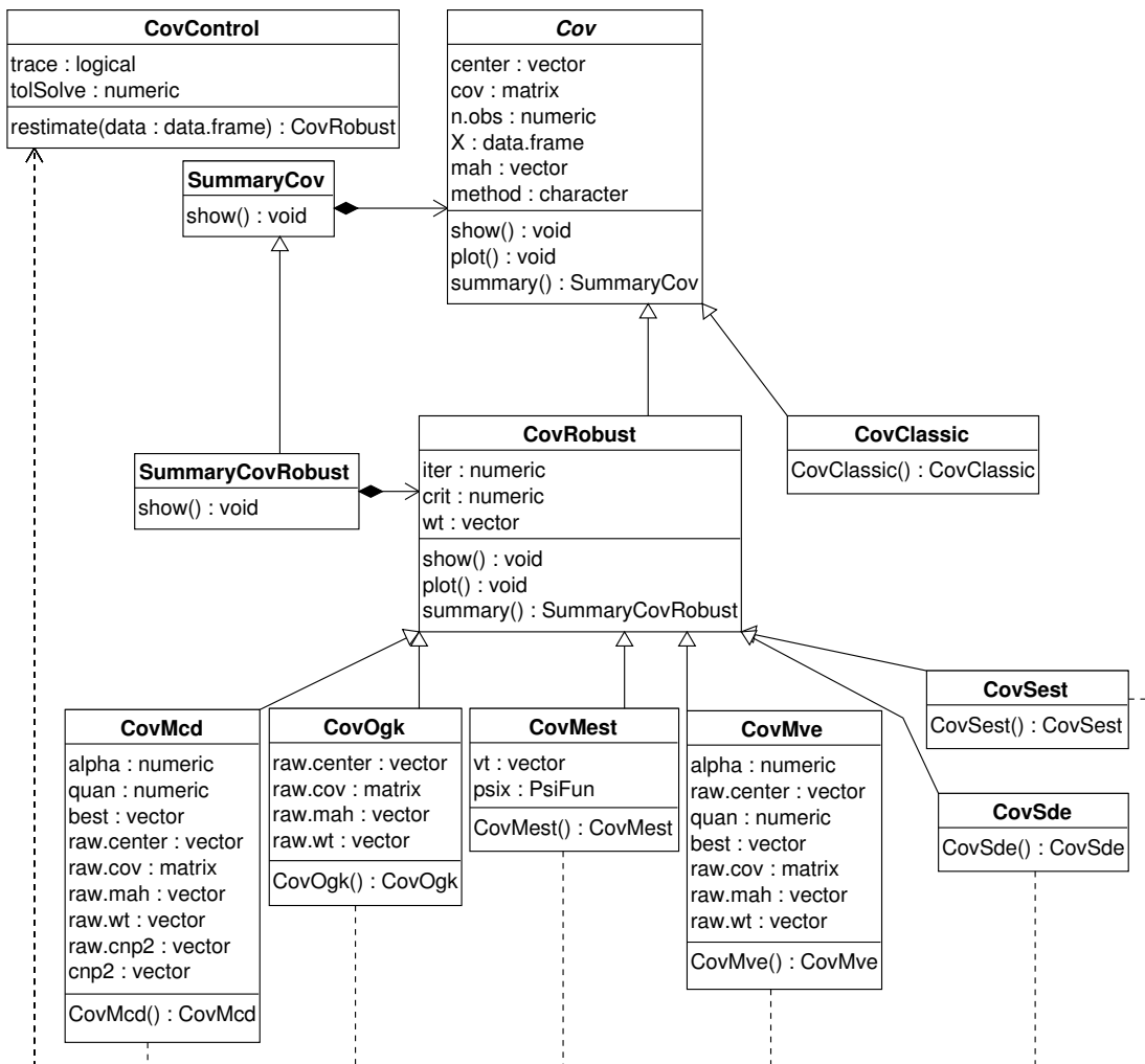
Figure 4: Object model for robust location and scatter estimation.
